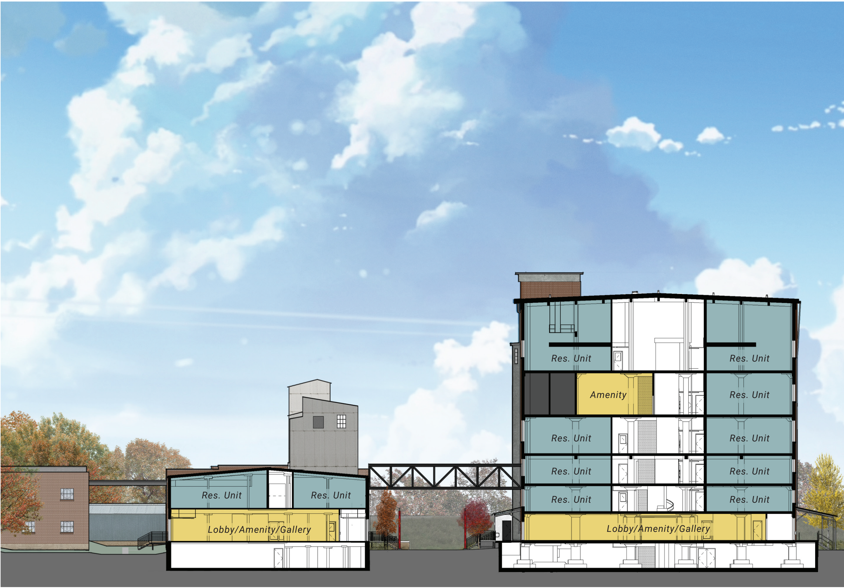
EAST-WEST SECTION - LOOKING NORTH Illustration by Cuningham Group
