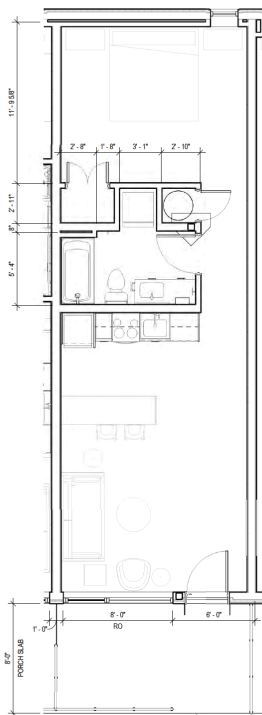
3 STUDIO - DIMENSION PLAN SCALE: 1/4" = 1'-0"
